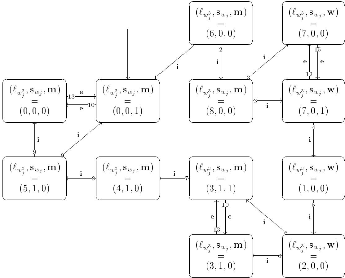
Figure 3.8: Transitions of \text{writer}_j^3 .
